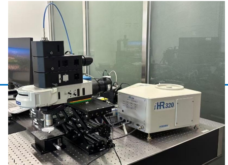
Custom Raman microscope based on Horiba
